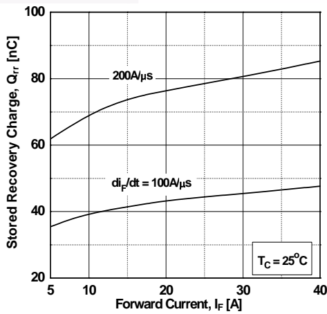
Figure 21. Stored Charge
