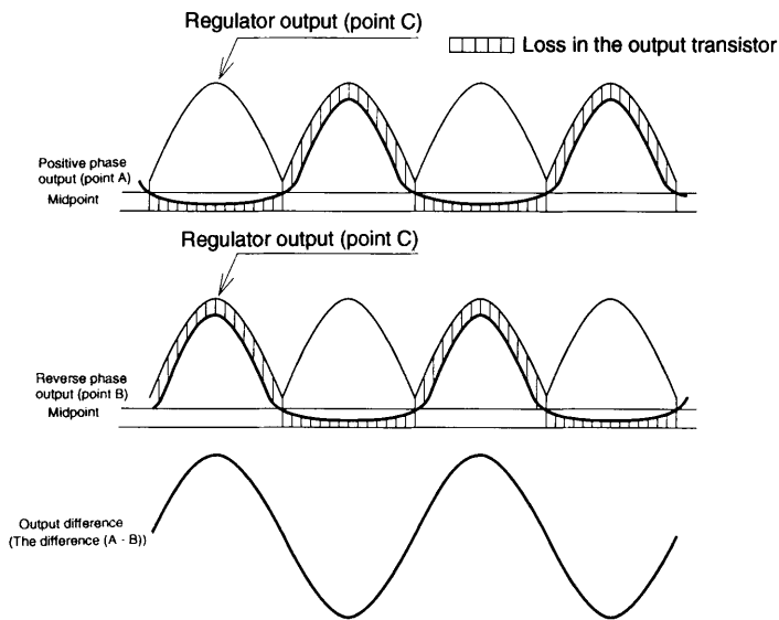
Figure 3 Output Waveforms
