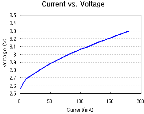
(1) Forward Voltage vs Forward Current
