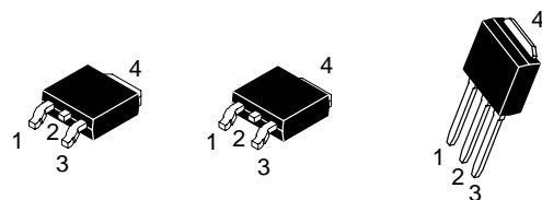
CASE 369AA DPAK (Surface Mount) STYLE 2
